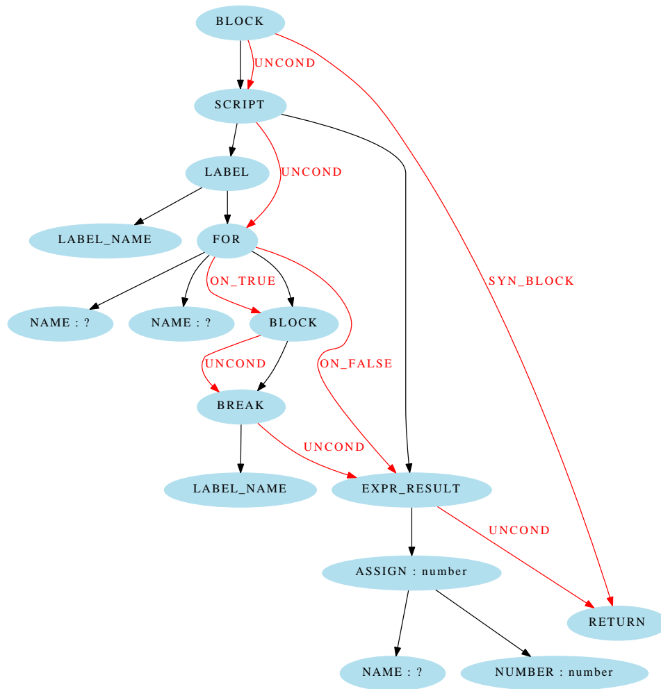
Figure 19: label: for (i in x) { break label; } i = 5;
