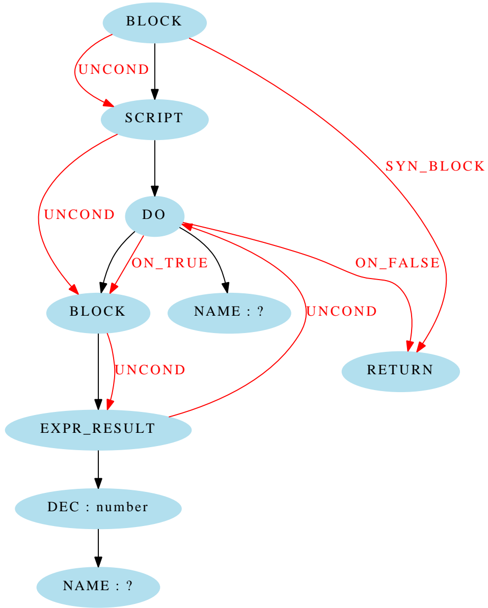
Figure 15: do { -x; } while (x);
